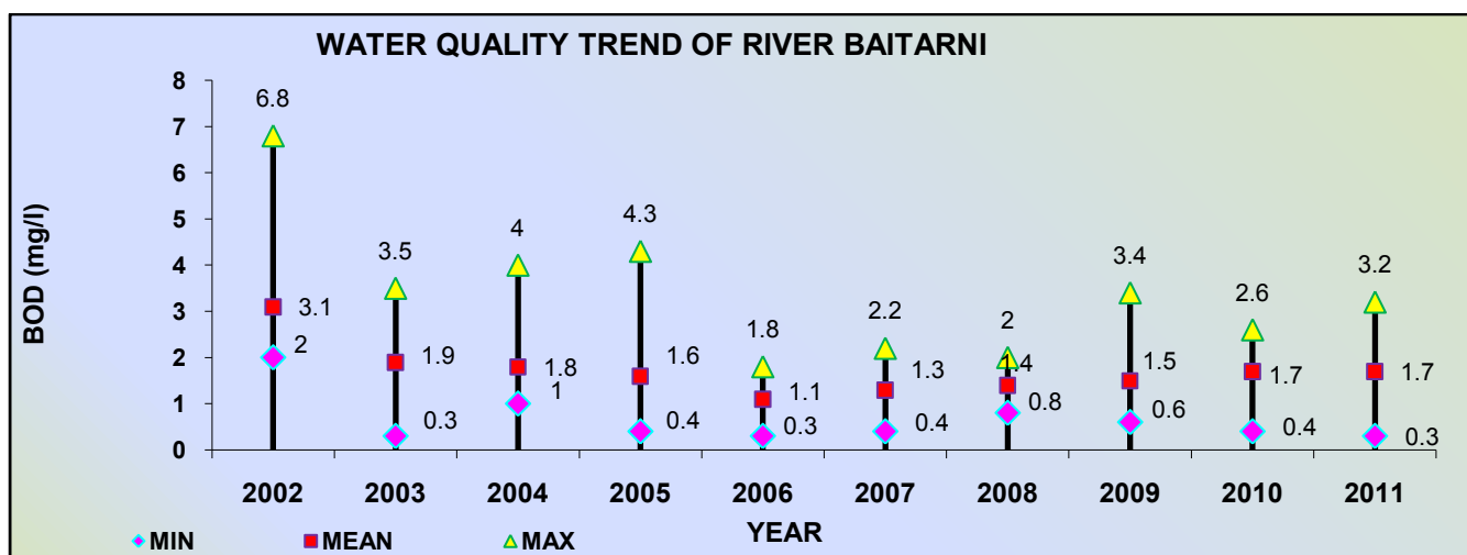
Figure 3.15: Water Quality Trend of BOD in River Baitarni
