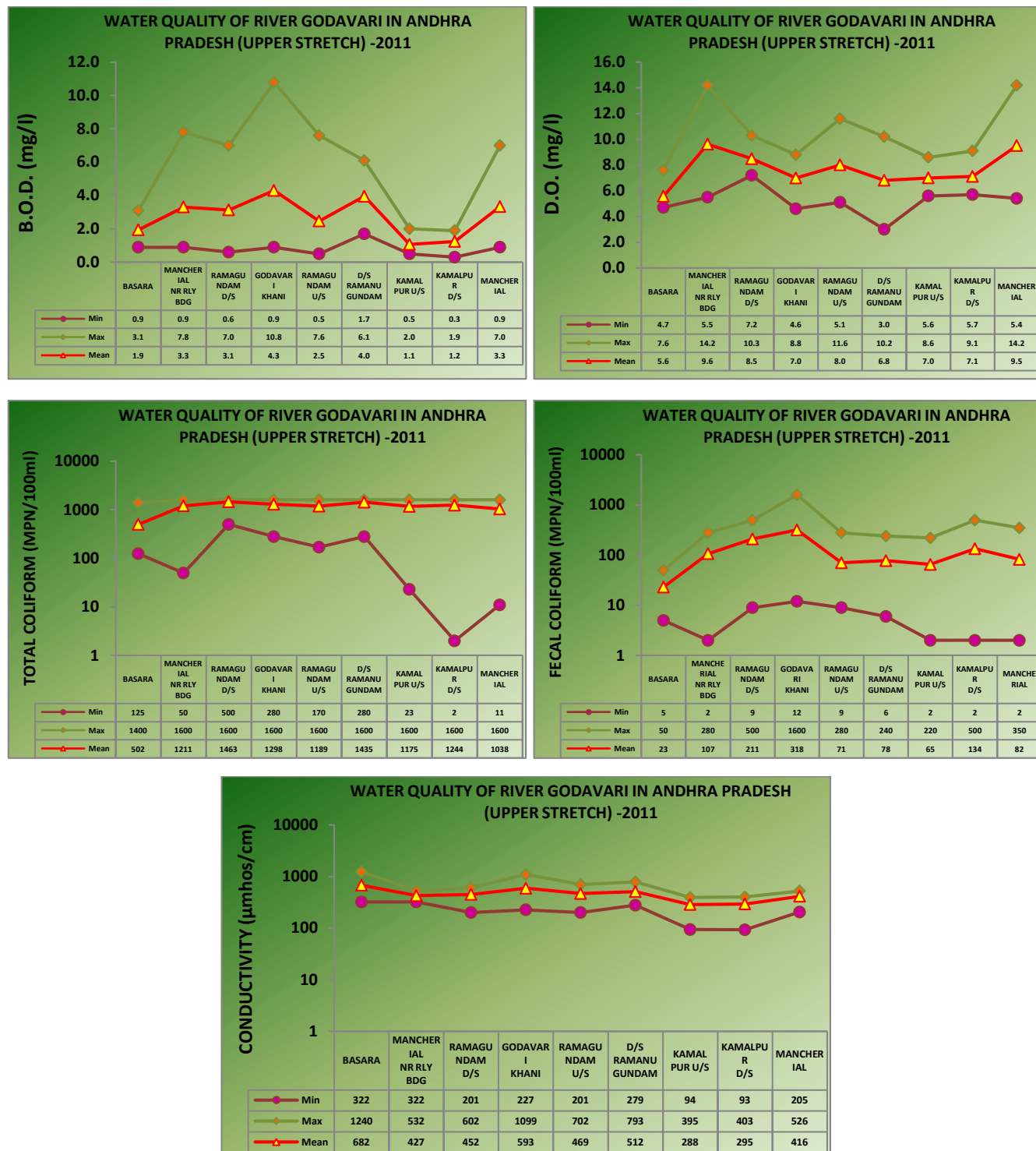
Figure 14.3: Water Quality of River Godavari in Andhra Pradesh (Upper Stretch)
