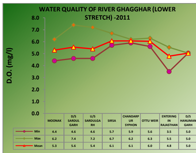
Figure 18.2: Water Quality of River Ghagghar (Lower Stretch)
