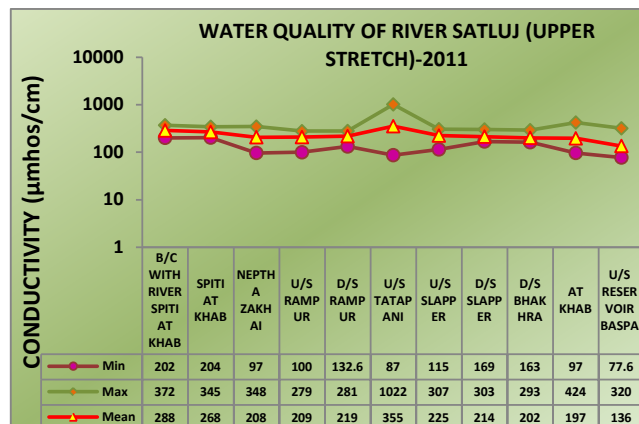
Figure 4.3: Water Quality of River Satluj (Upper Stretch)
