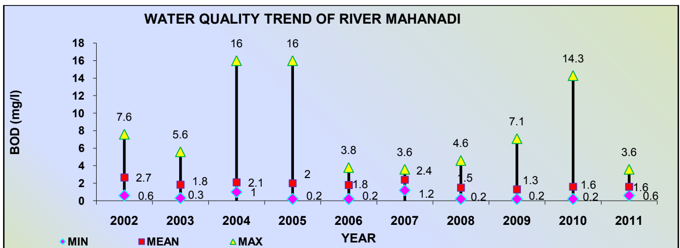
Figure 3.13: Water Quality Trend of BOD in River Mahanadi
