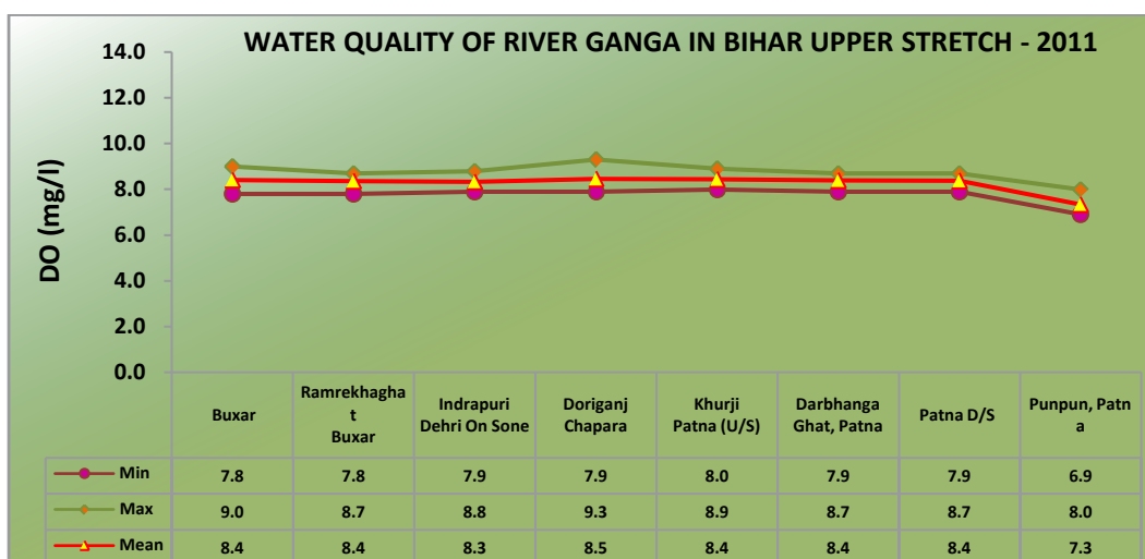
Figure 5.4: Water Quality of River Ganga in Bihar (Upper Stretch)
