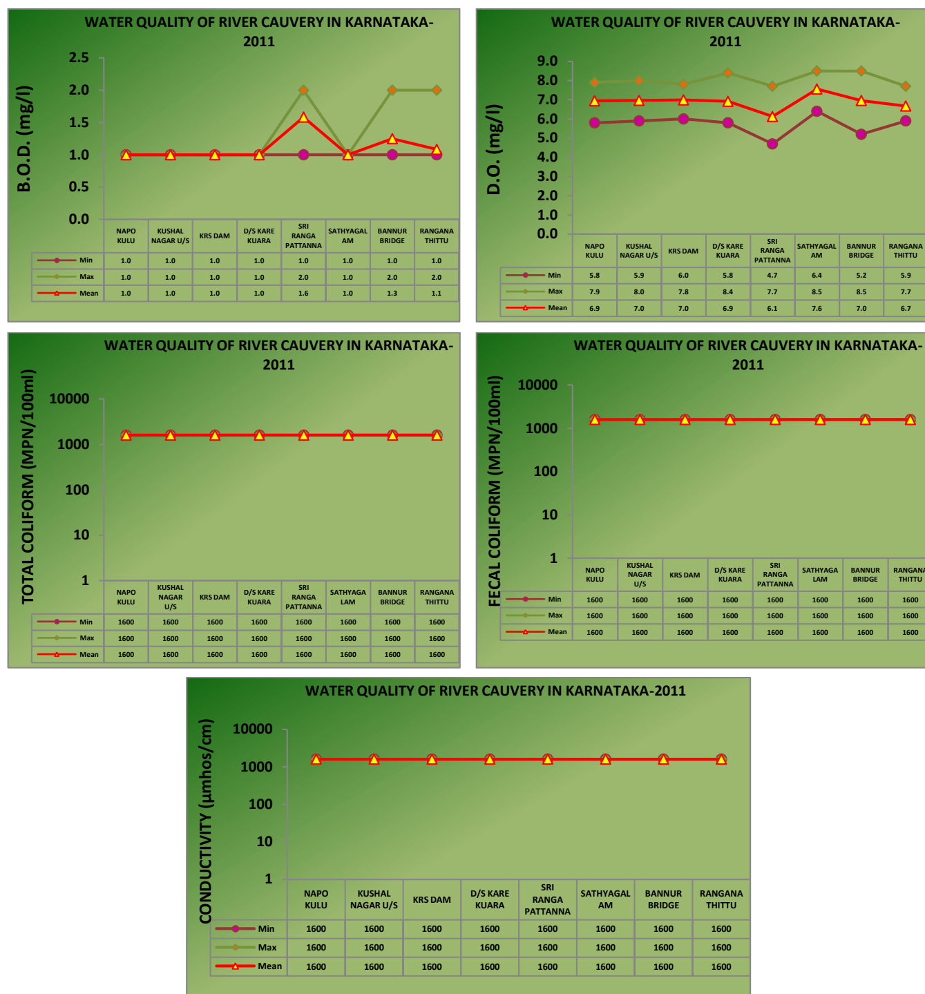
Figure 17.1: Water Quality of River Cauvery in Karnataka
