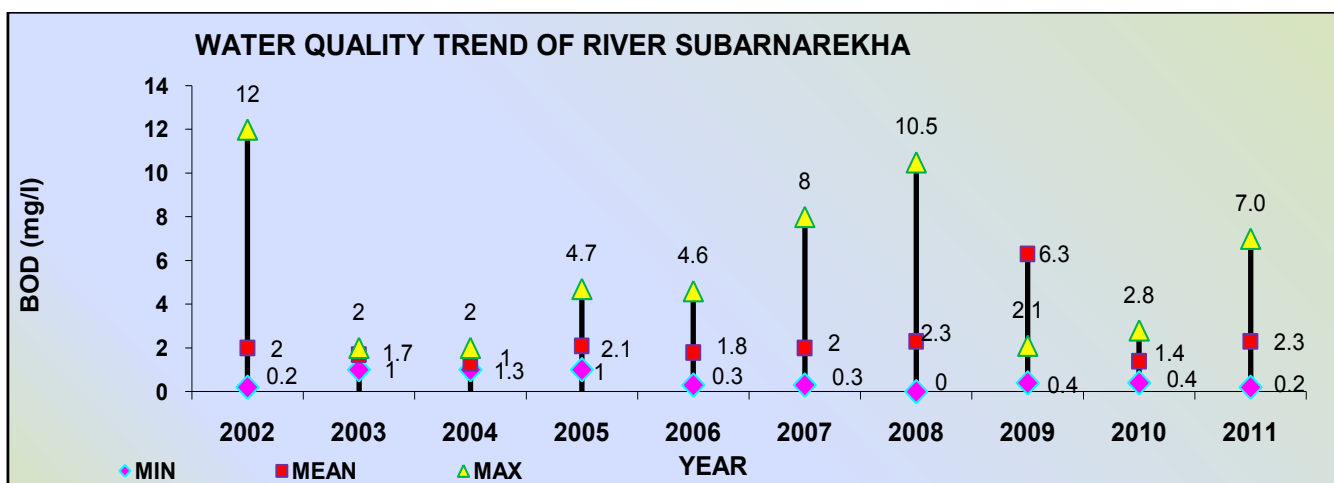
Figure 3.16: Water Quality Trend of BOD in River Subarnarekha
