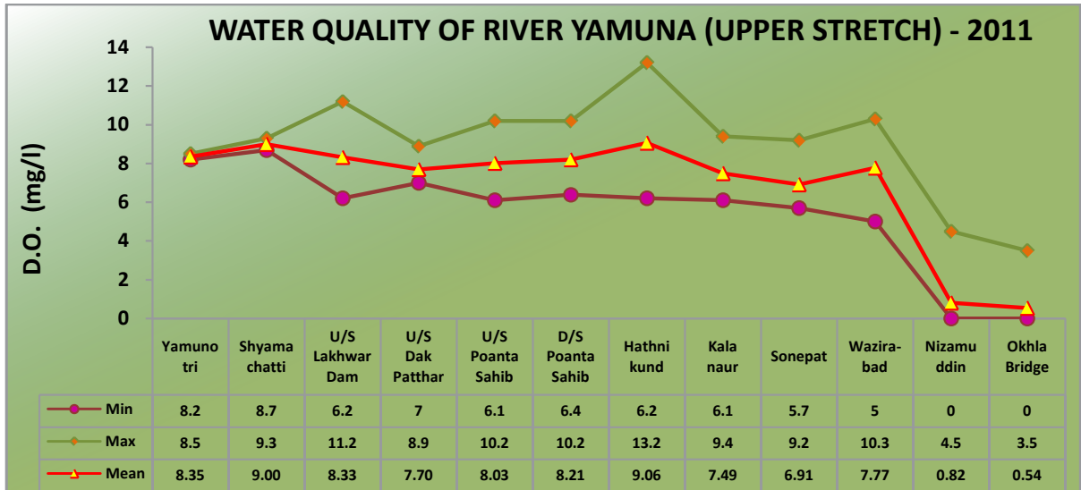
Figure 5.5: Water Quality of River Yamuna (Upper Stretch)
