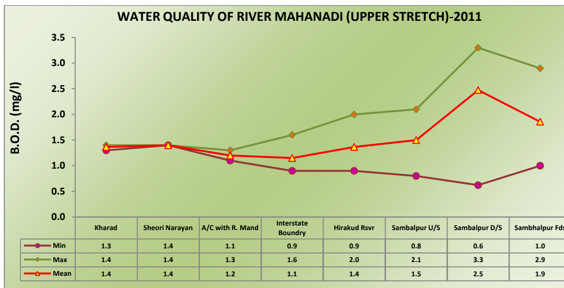
Figure 11.1: Water Quality of River Mahanadi (Upper Stretch)
