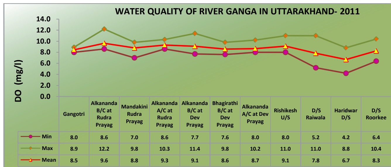
Figure 5.1: Water Quality of River Ganga in Uttarakhand
