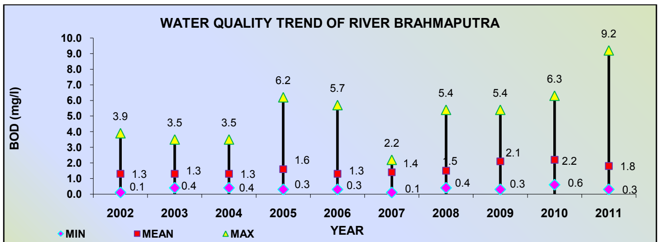
Figure 3.17: Water Quality Trend of BOD in River Brahmaputra
