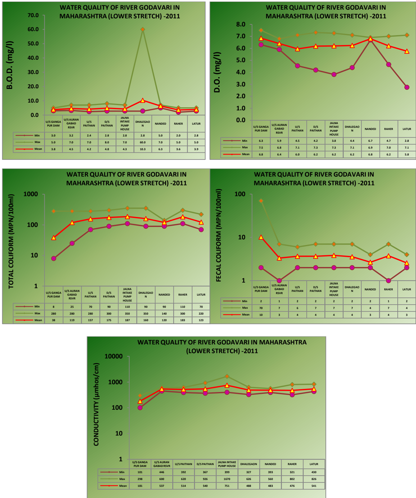
Figure 14.2: Water Quality of River Godavari in Maharashtra (Lower Stretch)
