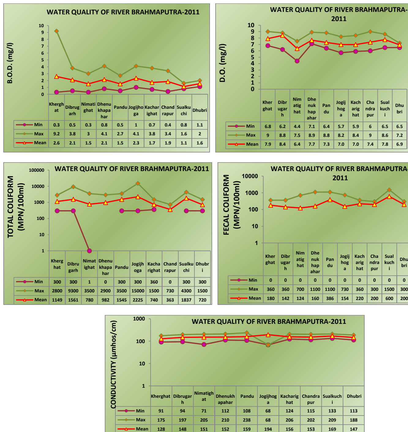
Figure 6.1: Water Quality of River Brahmaputra
