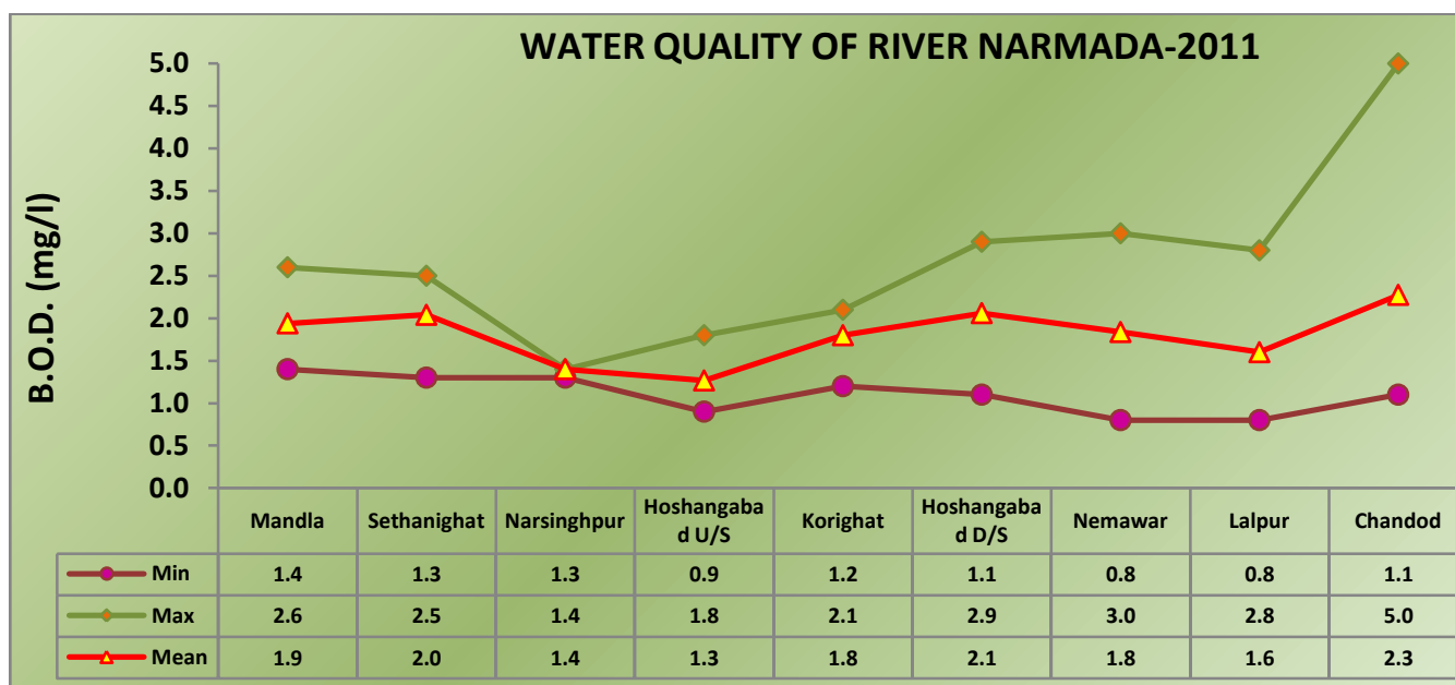
Figure 9.1: Water Quality of River Narmada
