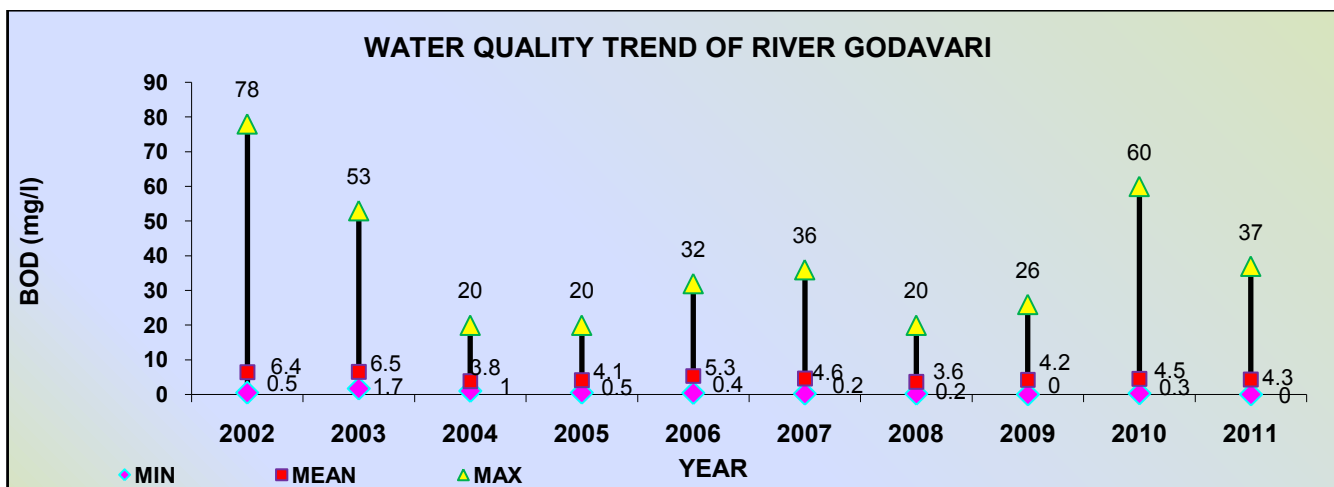
Figure 3.10: Water Quality Trend of BOD in River Godavari
