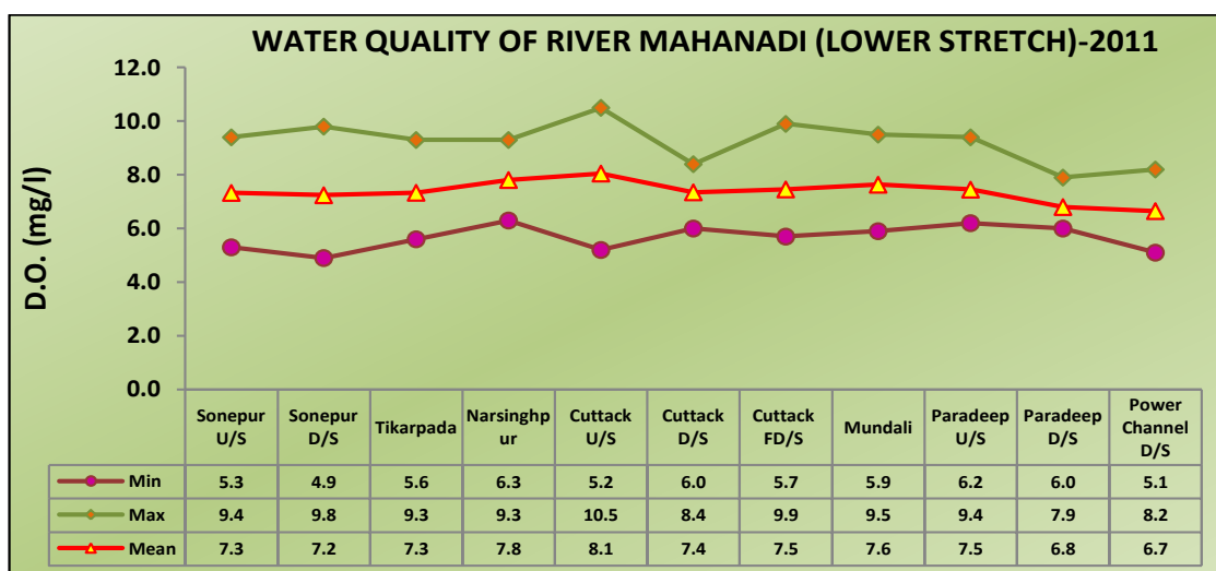
Figure 11.2: Water Quality of River Mahanadi (Lower Stretch)
