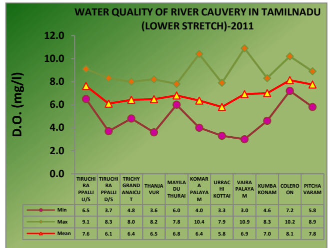
Figure 17.2: Water Quality of River Cauvery in Tamil Nadu (Lower Stretch)
