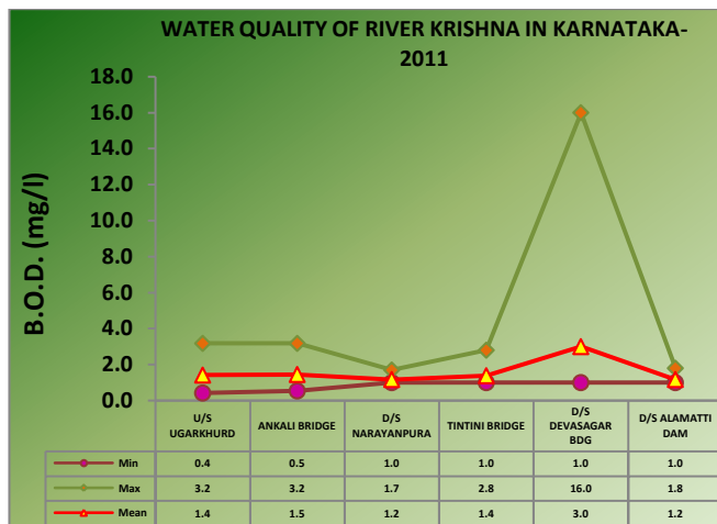
Figure 15.2: Water Quality of River Krishna in Karnataka
