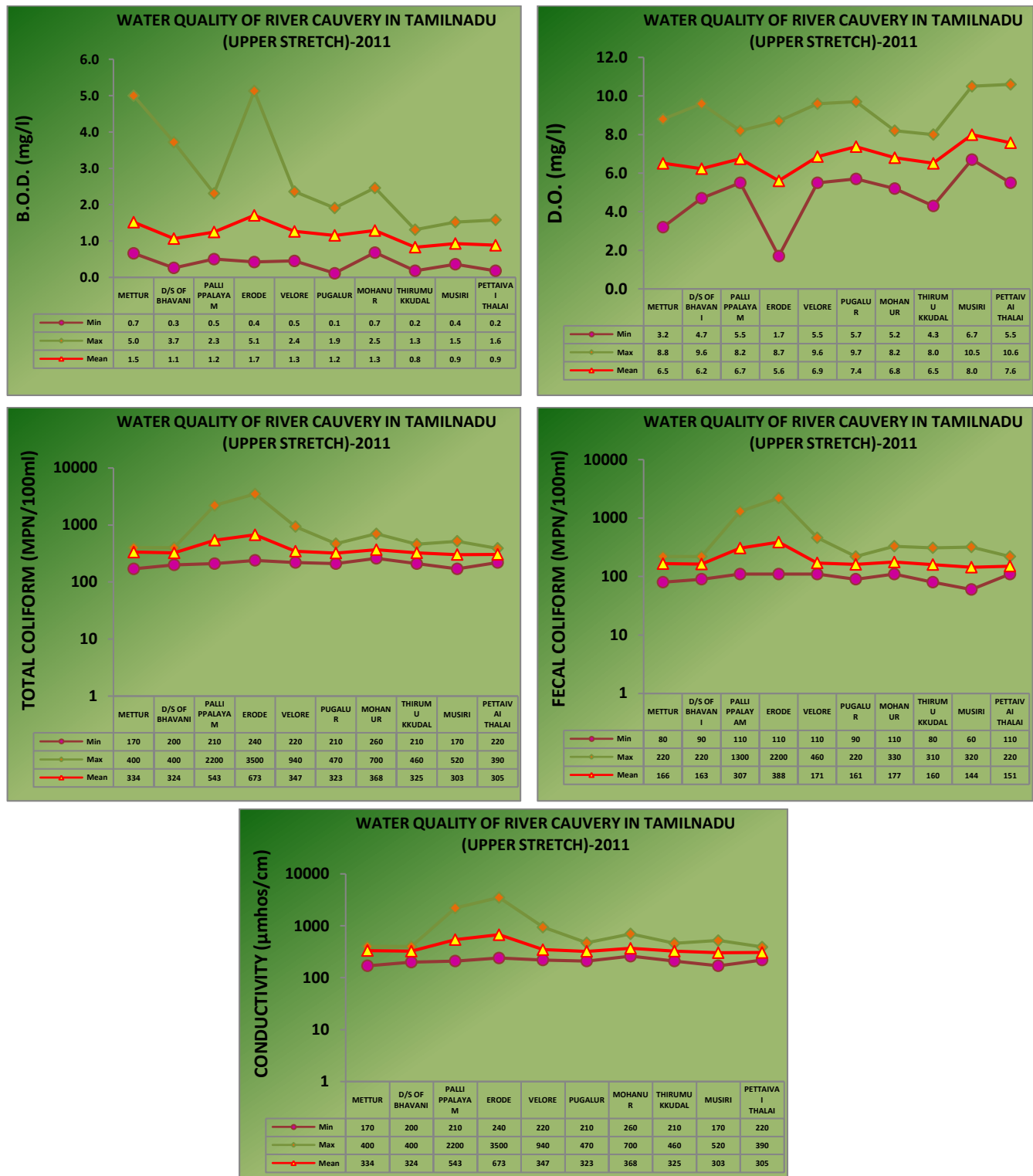
Figure 17.2: Water Quality of River Cauvery in Tamil Nadu (Upper Stretch)
