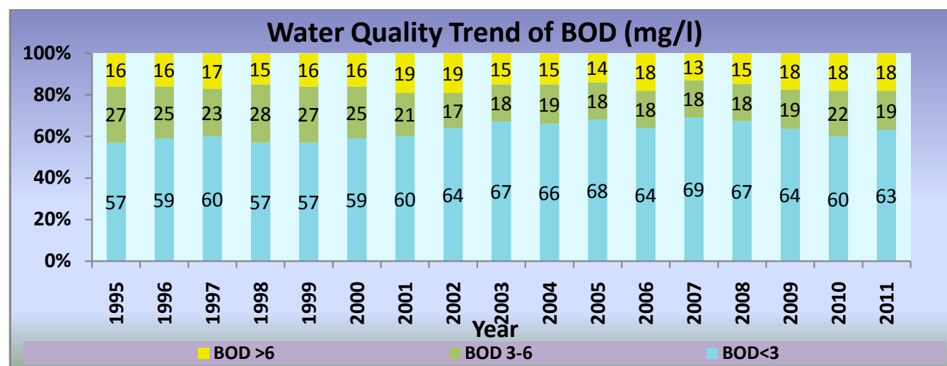
Figure 3.1 : Water Quality Trend (BOD, mg/l)
