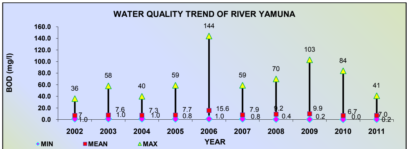
Figure 3.5: Water Quality Trend of BOD in River Yamuna
