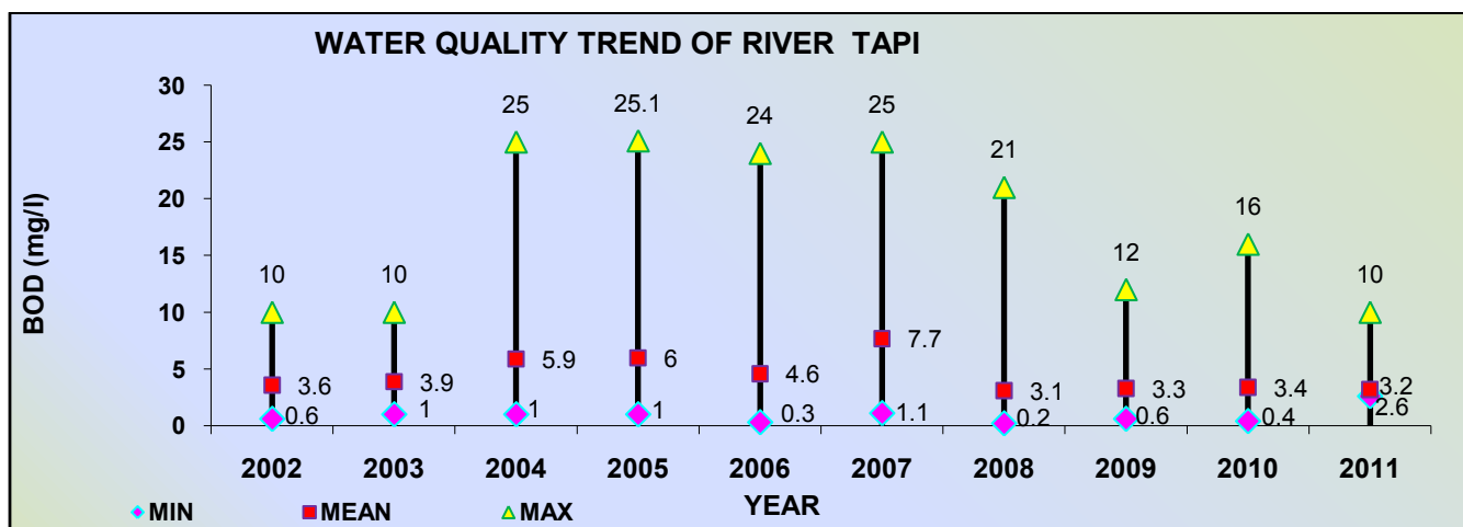
Figure 3.8: Water Quality Trend of BOD in River Tapi
