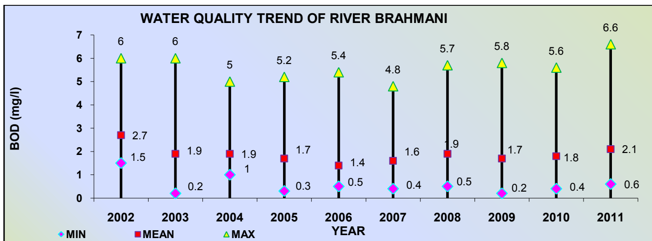
Figure 3.14: Water Quality Trend of BOD in River Brahmani
