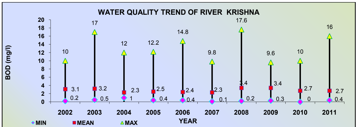
Figure 3.11: Water Quality Trend of BOD in River Krishna
