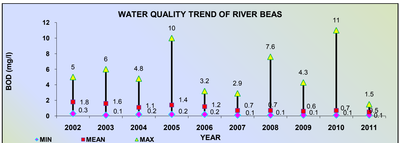
Figure 3.19: Water Quality Trend of BOD in River Beas
