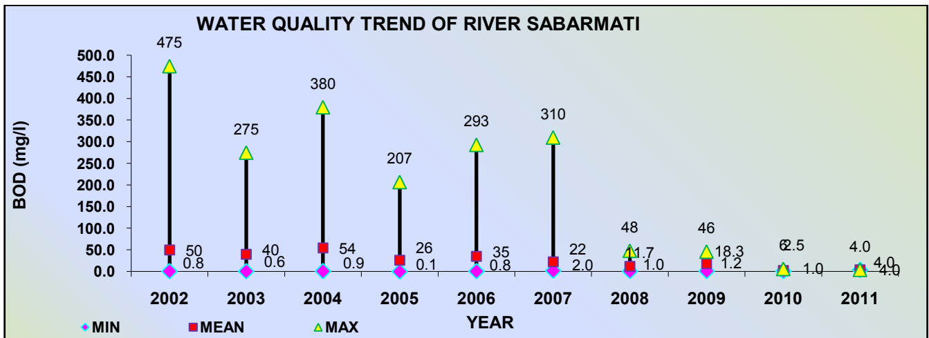
Figure 3.6: Water Quality Trend of BOD in River Sabarmati
