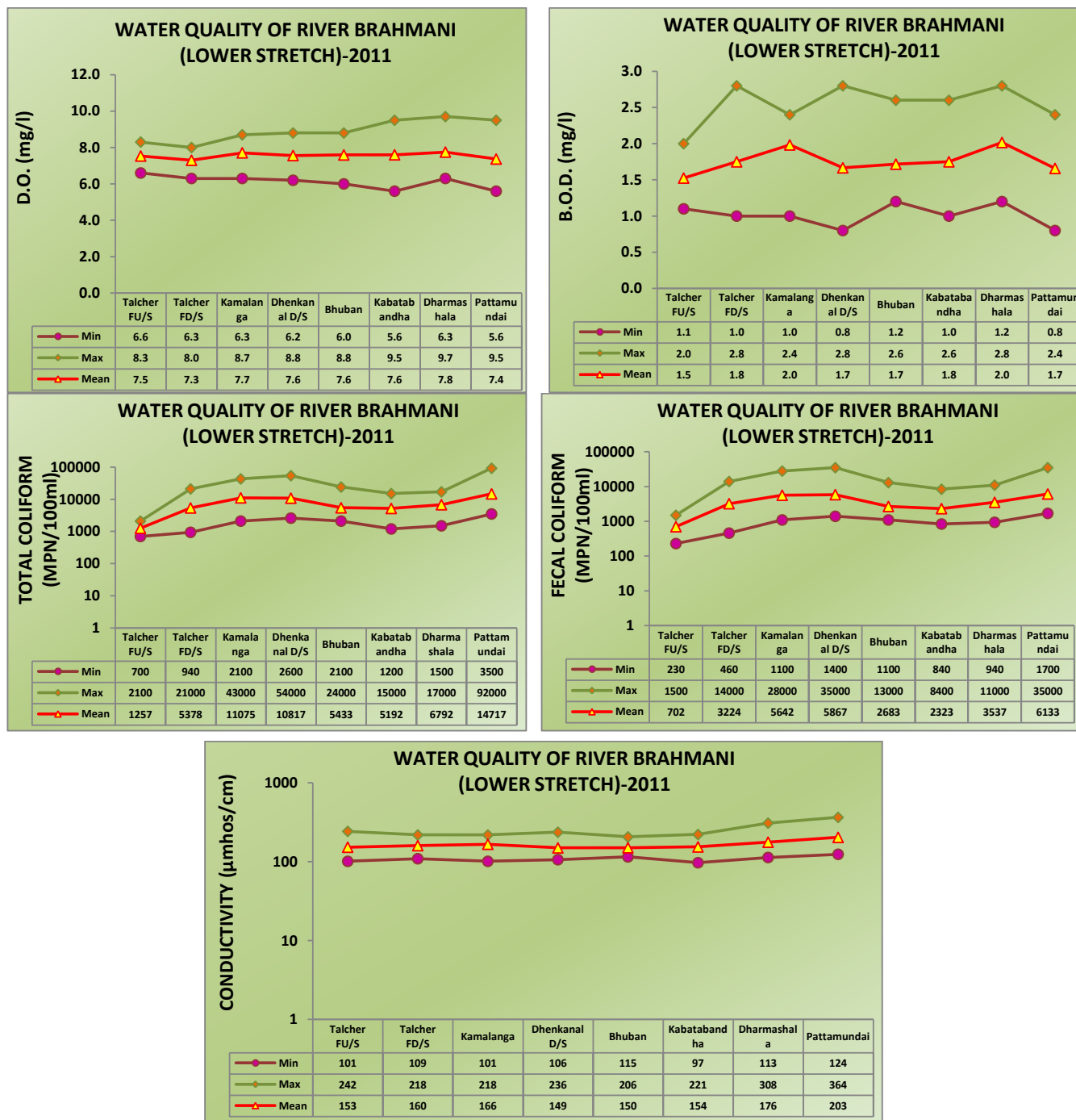
Figure 12.2: Water Quality of River Brahmani (Lower Stretch)
