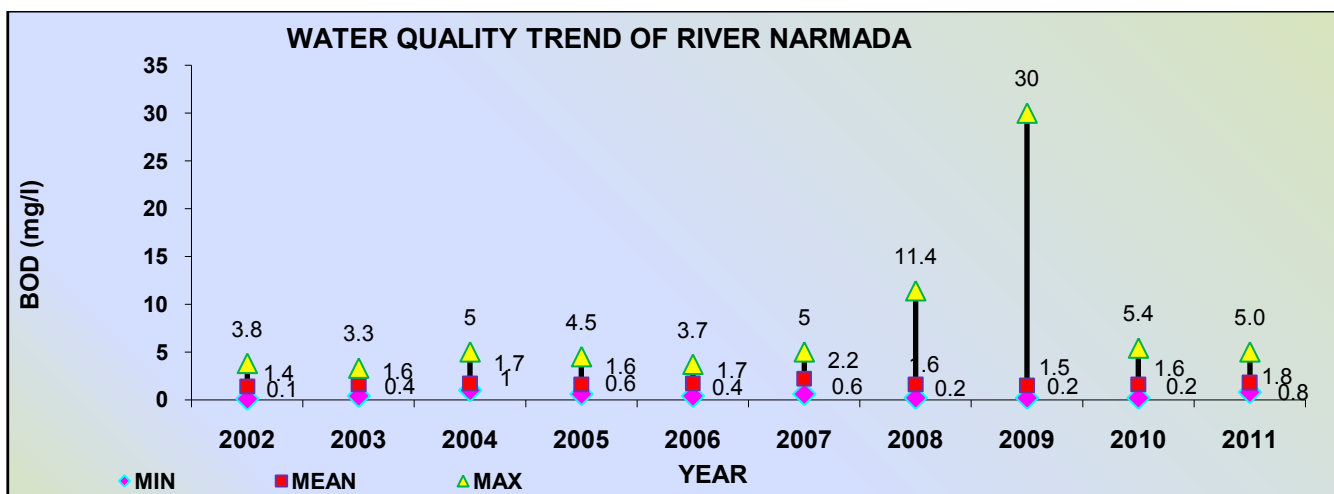
Figure 3.9: Water Quality Trend of BOD in River Narmada
