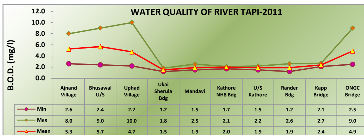
Figure 10.1: Water Quality of River Tapi
