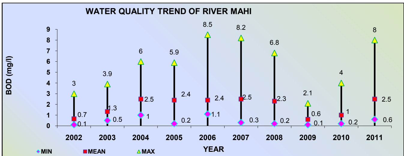
Figure 3.7: Water Quality Trend of BOD in River Mahi
