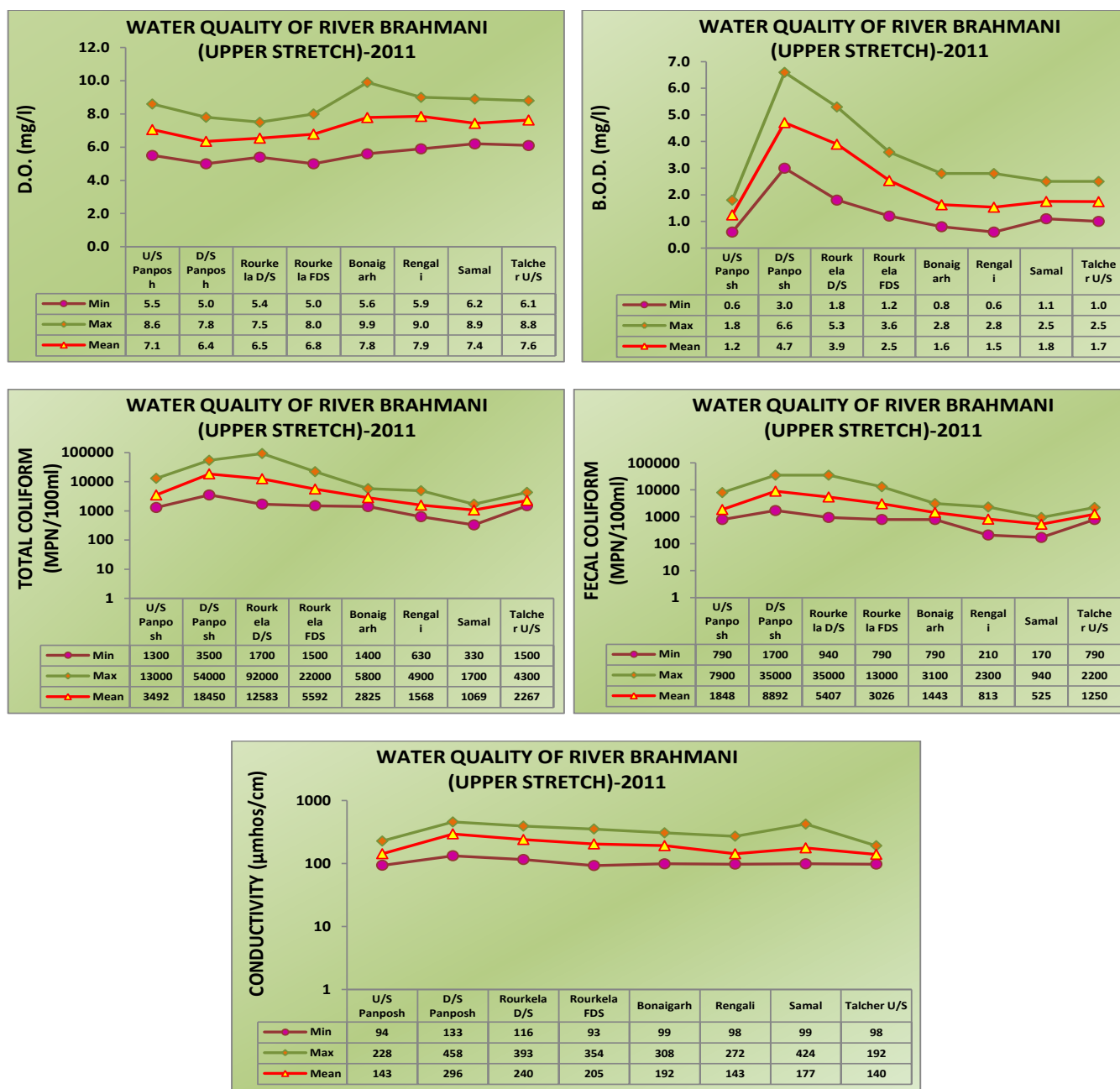
Figure 12.1: Water Quality of River Brahmani (Upper Stretch)
