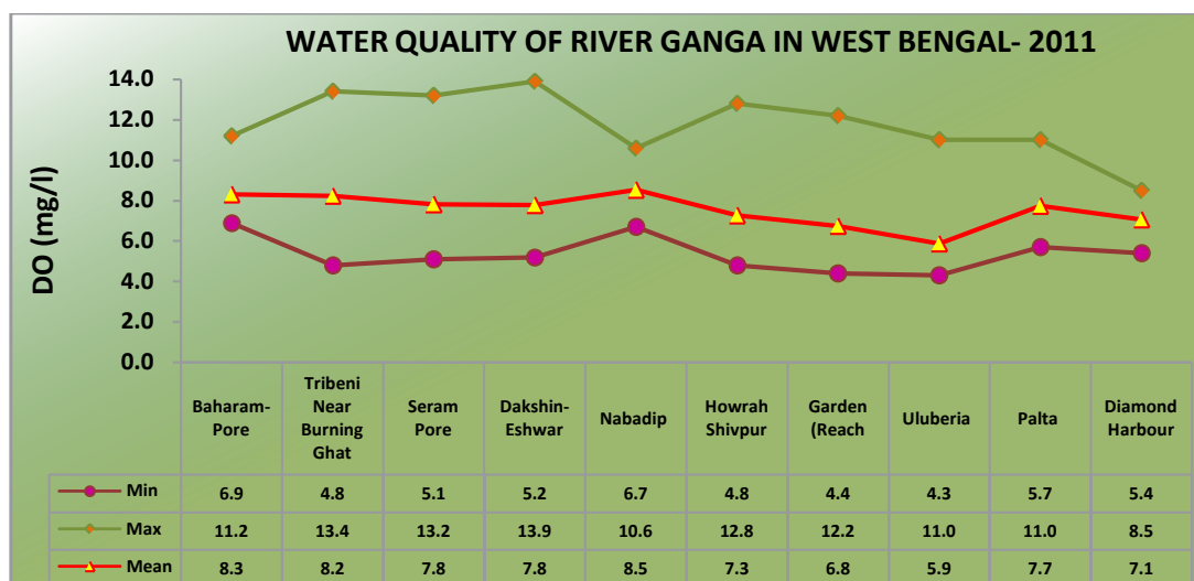
Figure 5.6: Water Quality of River Ganga in West Bengal
