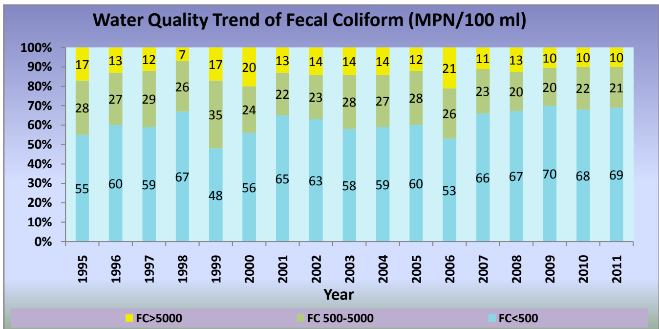
Figure 3.3 : Water Quality Trend (Faecal Colliform, MPN/100 ml)
