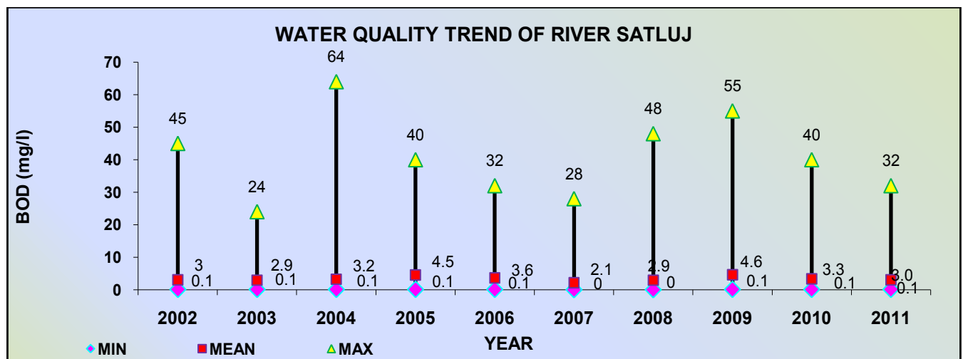
Figure 3.18: Water Quality Trend of BOD in River Satluj
