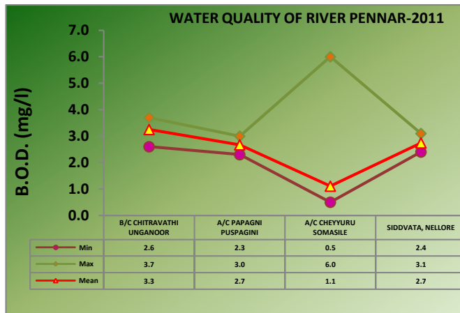
Figure 16.1: Water Quality of River Pennar
