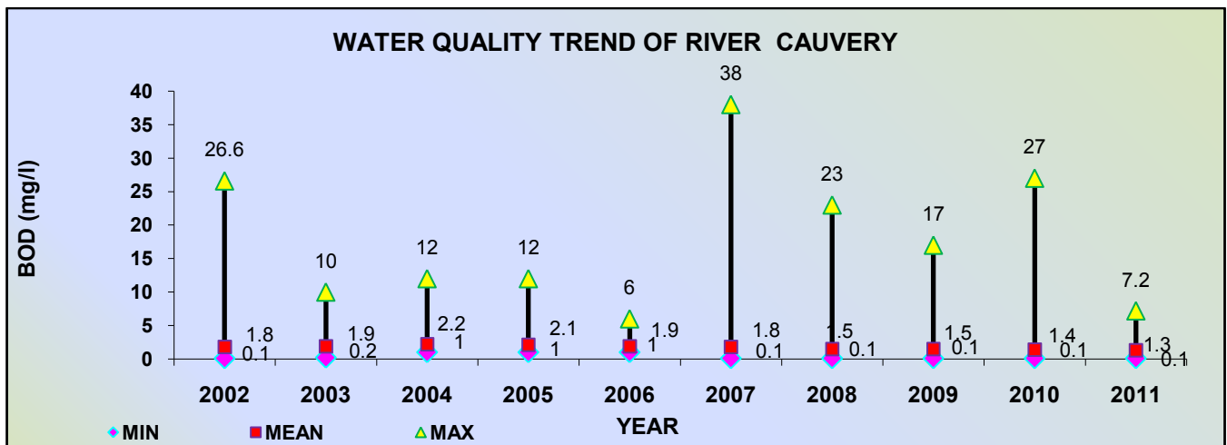
Figure 3.12: Water Quality Trend of BOD in River Cauvery
