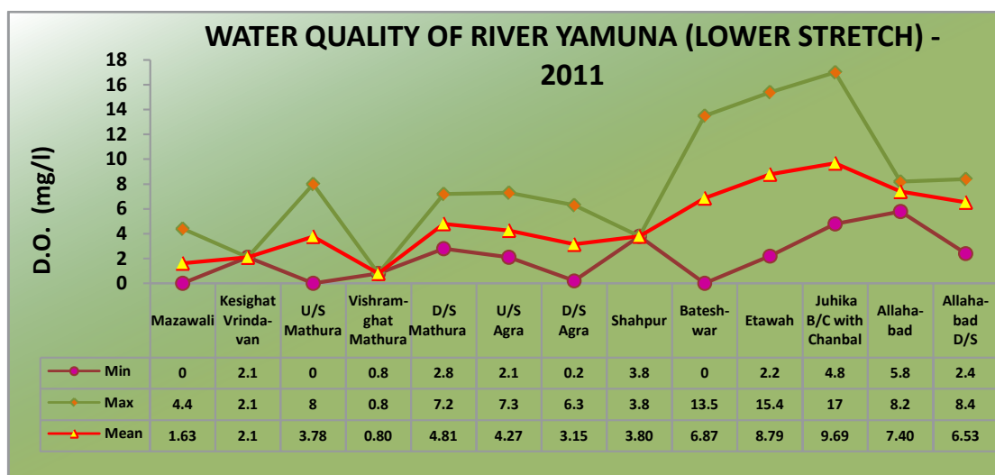
Figure 5.6: Water Quality of River Yamuna (Lower Stretch)
