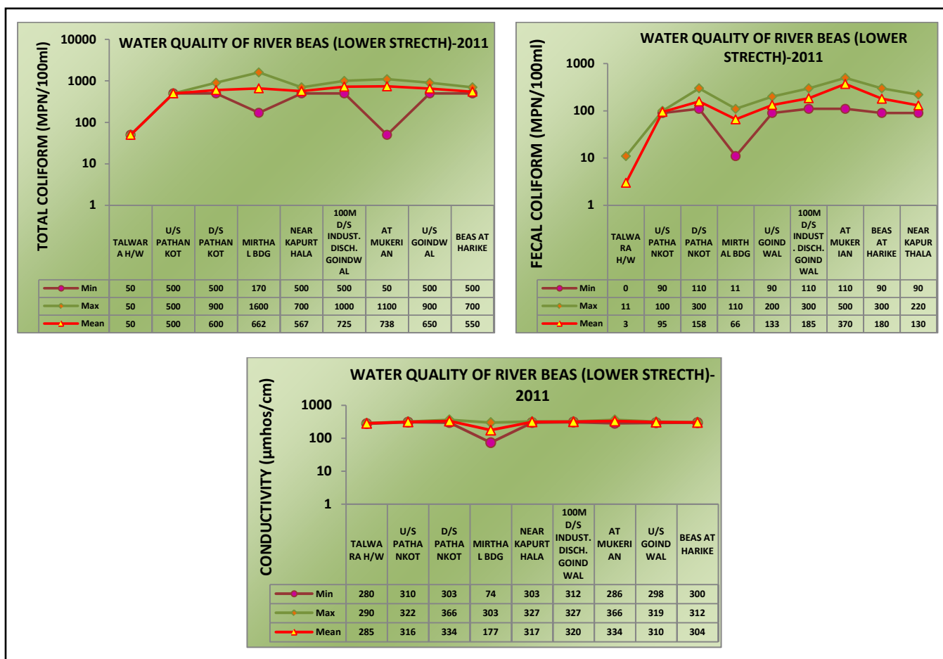
Figure 4.2: Water Quality of River Beas (Lower Stretch)
