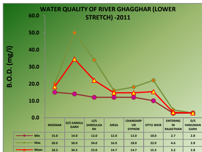
Figure 18.2: Water Quality of River Ghagghar (Lower Stretch)
