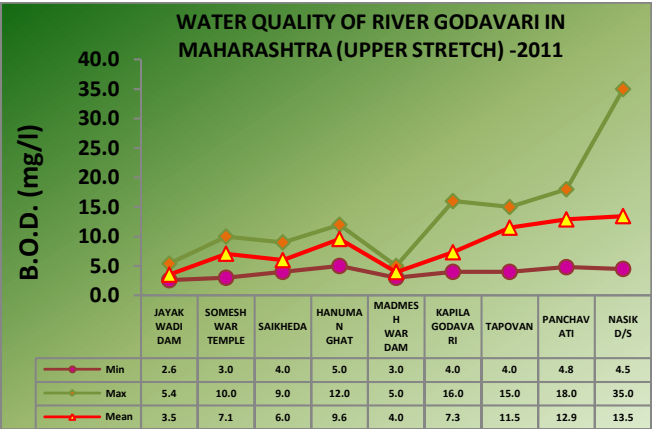
Figure 14.1: Water Quality of River Godavari in Maharashtra (Upper Stretch)
