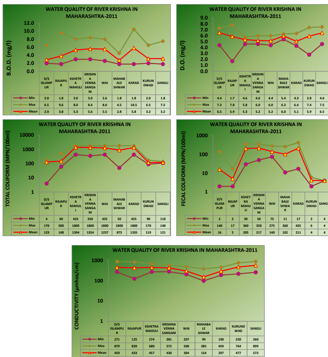
Figure 15.1: Water Quality of River Krishna in Maharashtra
