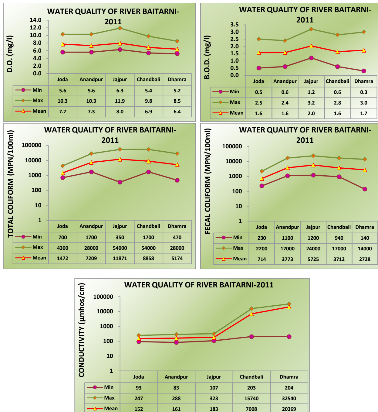
Figure 12.3: Water Quality of River Baitarni
