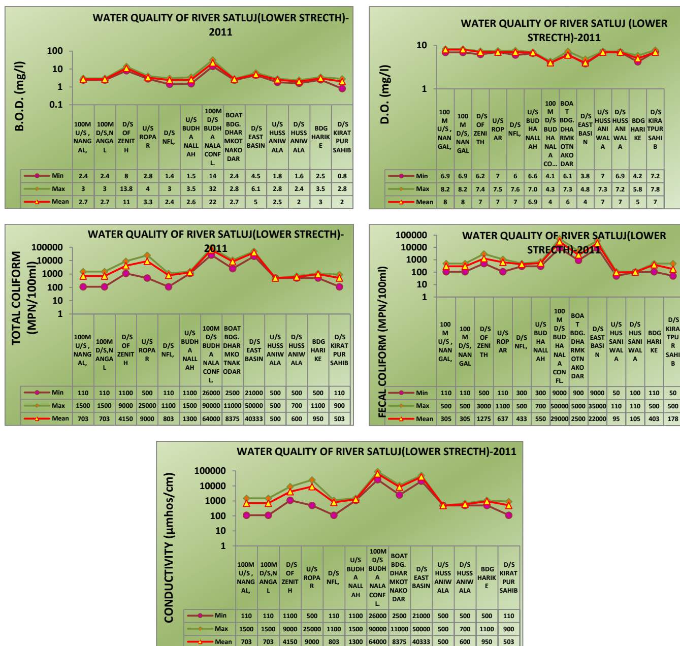
Figure 4.4: Water Quality of River Satluj (Lower Stretch)
