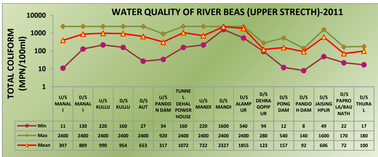
Figure 4.1: Water Quality of River Beas (Upper Stretch)
