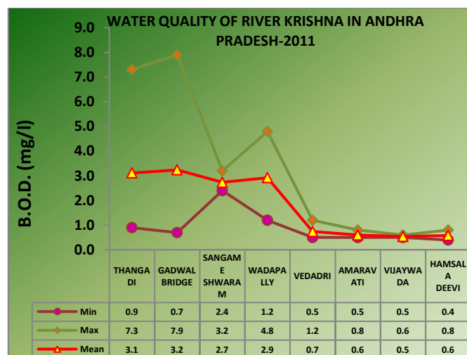
Figure 15.3: Water Quality of River Krishna in Andhra Pradesh
